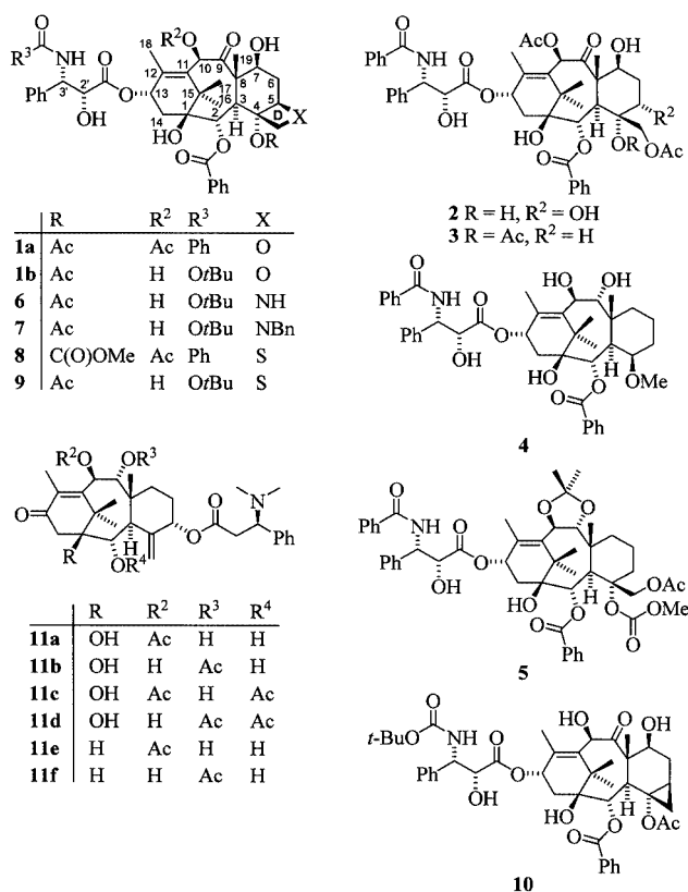
Figure 1. Structures of paclitaxel ( 1a ), docetaxel ( 1b ), paclitaxel analogues 2–10 , and taxines 11a–11f
