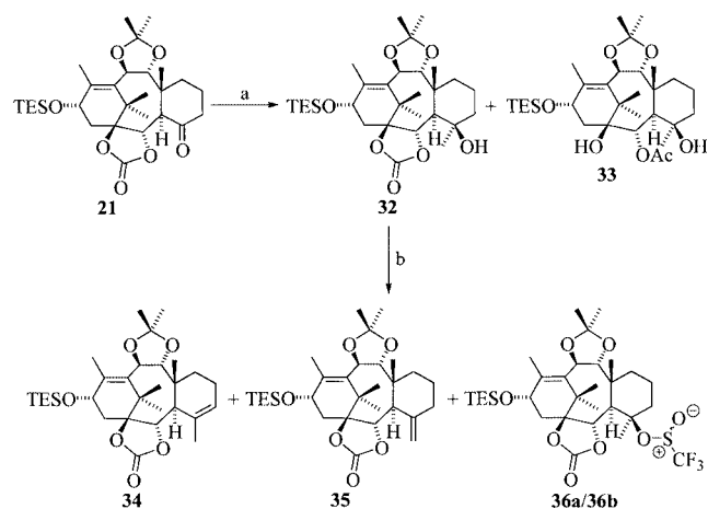
Scheme 6. Conversion of 21 into a mixture of 34 and 35 , 36a , and 36b ; reagents and conditions: (a) MeLi, THF, –78 °C, 15 min, 32 : 82%, 33 : 4%; (b) CF 3 SO 2 Cl, DMAP, CH 2 Cl 2 , 2 d, 34/35 (10:1 mixture): 19%, 36a/36b : 32% and 29%
