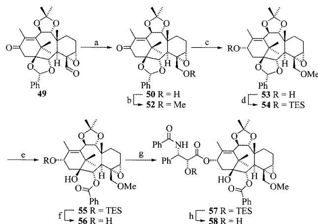
Scheme 10. Conversion of 49 into paclitaxel derivative 58 ; reagents and conditions: (a) NaBH 4 , MeOH, 0 °C, 1 h, 77%; (b) NaH, MeI, THF, 3 h, 69%; (c) NaBH 4 , CeCl 3 , MeOH, 0 °C, 30 min, 73%; (d) TESCl, imidazole, DMF, 2 h, 97%; (e) t BuOOH, Pd(OAc) 2 , toluene, 70 °C, 20 h, 35%; (f) TBAF, THF, 15 min, 85%; (g) 28 , NaHMDS, THF, -78 °C, 1 h, 49%; (h) TBAF, THF, 5 min, 81%
