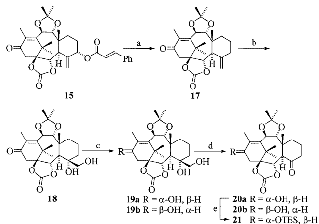
Scheme 3. Preparation of key intermediate 21 from 15 ; reagents and conditions: (a) \text{HCOOH} , \text{NEt}_3 , \text{Pd}(\text{dba})_2 , \text{PPh}_3 , THF, reflux, 2 d, 97%; (b) \text{OsO}_4 , NMO, THF/ \text{H}_2\text{O} , 5 d, 91%; (c) \text{NaBH}_4 , \text{CeCl}_3 , MeOH, 0 °C, 30 min; (d) \text{NaIO}_4 , THF/ \text{H}_2\text{O} , 3 h, 20a : 49% (2 steps), 20b : 12% (2 steps); (e) \text{TESCl} , imidazole, DMF, 4 h, 86%
