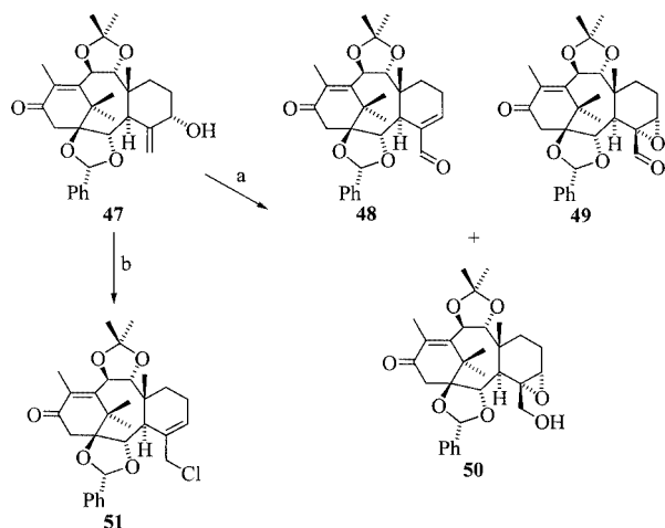
Scheme 9. Conversion of 47 into 48 – 50 and 51 by PCC oxidation and Swern oxidation, respectively; reagents and conditions: (a) PCC, CH 2 Cl 2 , 3.5 h; 48 : 5%, 49 : 43%, 50 : 2%; (b) (COCl) 2 , DMSO, CH 2 Cl 2 , -50 °C, 10 min, then 47 , -10 °C, 20 min, then Et 3 N, -10 °C → room temp., 40 min, 21%
