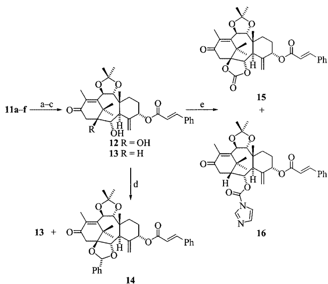
Scheme 2. Conversion of taxines 11 into 13 and 14 , and into 15 and 16 ; reagents and conditions: (a)–(d) ref. [9] ; (e) CDI, butanone, reflux, 3 h, 15 : 86%, 16 : 9%
