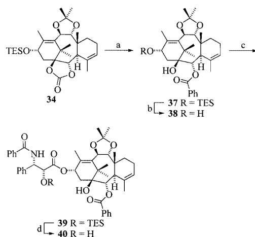
Scheme 7. Preparation of paclitaxel analogue 40 from 34 ; reagents and conditions: (a) PhLi, THF, -78^{\circ}\text{C} , 30 min, 80%; (b) TBAF, THF, 5 min, 84%; (c) 28 , NaHMDS, THF, -78^{\circ}\text{C} , 20 min, 66%; (d) TBAF, THF, 5 min, 79%
