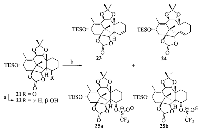
Scheme 4. Preparation of compounds 23 , 24 , 25a , and 25b from 21 ; reagents and conditions: (a) \text{NaBH}_4 , MeOH, 0 °C, 30 min; (b) (I) (\text{CF}_3\text{SO}_2)_2\text{O} , pyridine, \text{CH}_2\text{Cl}_2 , 2 d, 23/24 (1:10 mixture): 34%, 25a/25b : 16% and 4%, or (II) \text{CF}_3\text{SO}_2\text{Cl} , DMAP, \text{CH}_2\text{Cl}_2 , 2 d, 23/24 (9:1 mixture): 31%, 25a/25b : 17% and 4%
