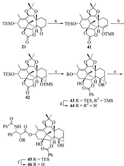
Scheme 8. Preparation of paclitaxel analogue 46 from 21 ; reagents and conditions: (a) LDA, TMSCl, THF, -78^{\circ}\text{C} \rightarrow -20^{\circ}\text{C} , 1 h, 92%; (b) \text{CH}_2\text{I}_2 , Zn/Cu, \text{Et}_2\text{O}/\text{DME} , 50^{\circ}\text{C} , 60 h, 58%; (c) PhLi, THF, -78^{\circ}\text{C} , 2.5 h, 86%; (d) TBAF, THF, 30 min, 58%; (e) 28 , NaHMDS, THF, -78^{\circ}\text{C} , 45 min, 45%; (f) TBAF, THF, 5 min, 76%
