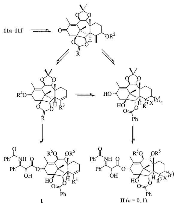
Scheme 1. General scheme for the preparation of paclitaxel derivatives I and II
