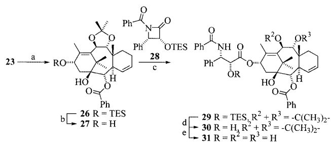
Scheme 5. Preparation of paclitaxel derivatives 30 and 31 from 23 ; reagents and conditions: (a) PhLi, THF, –78 °C, 30 min, 100%; (b) TBAF, THF, 5 min, 95%; (c) 28 , NaHMDS, THF, –78 °C, 20 min, 84%; (d) TBAF, THF, 5 min, 92%; (e) PTSA, MeOH, 3 h, 80%
