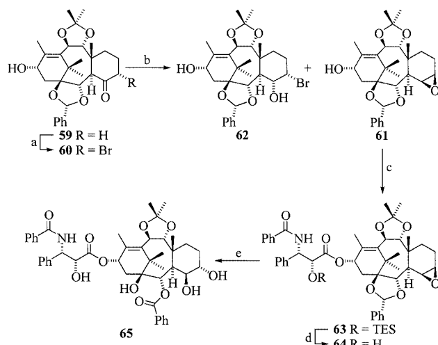
Scheme 11. Conversion of 59 into paclitaxel derivative 65 ; reagents and conditions: (a) PTAB, THF, -15\text{ }^{\circ}\text{C} \rightarrow 10\text{ }^{\circ}\text{C} , 3 h, 77%; (b) \text{NaBH}_4 , THF/MeOH, 0\text{ }^{\circ}\text{C} , 2 h, 61 : 36%, 62 : 31%; (c) 28 , NaHMDS, THF, -78\text{ }^{\circ}\text{C} , 1 h, 74%; (d) TBAF, THF, 5 min, 96%; (e) t\text{BuOOH} , \text{Pd}(\text{OAc})_2 , toluene, 70\text{ }^{\circ}\text{C} , 40 h, 17%
